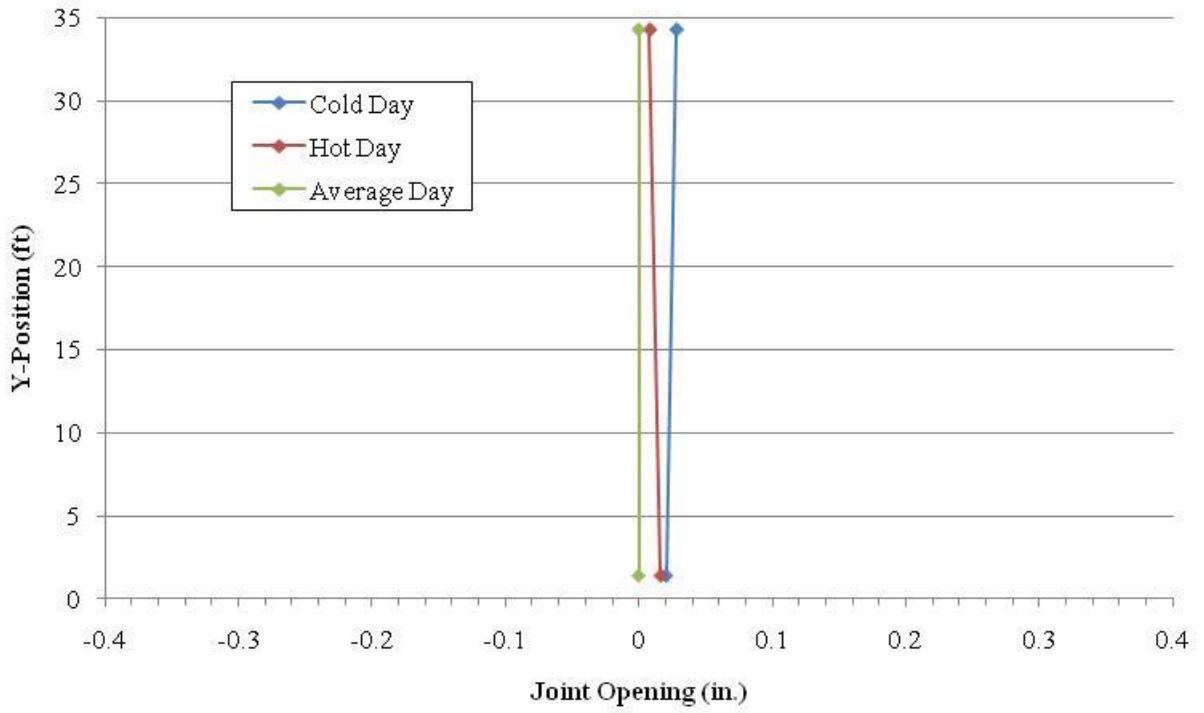
Figure 4.27. Abutment joint opening across approach slab for cold day, hot day and an average day
