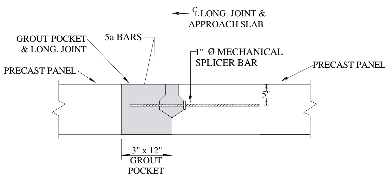
Figure 3.4. Longitudinal joint at centerline of approach slab at location of mechanical splicer bar (Bierwagen 2009)
