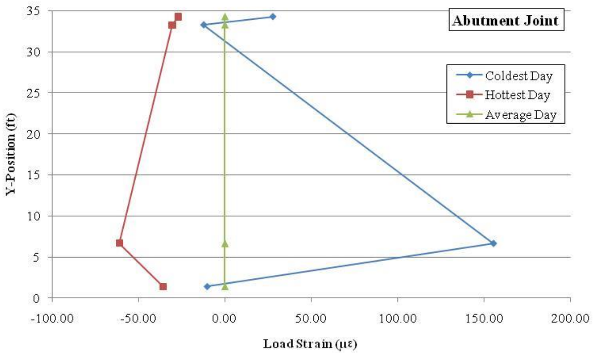
Figure 4.16. Load strain across the abutment joint of the approach slab for the cold, hot, and average days
