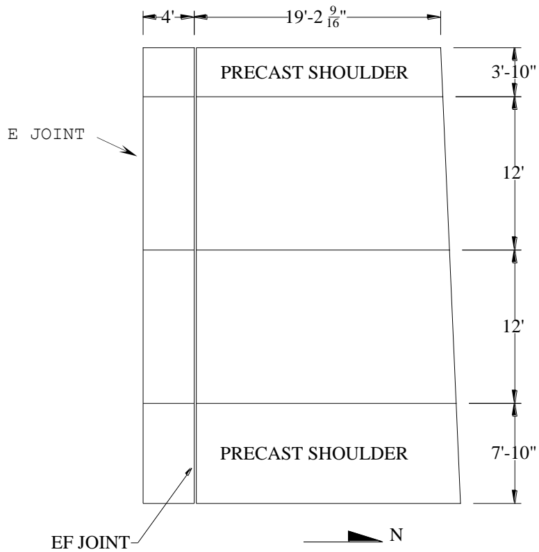
Figure 3.2. Plan view of precast approach slab
