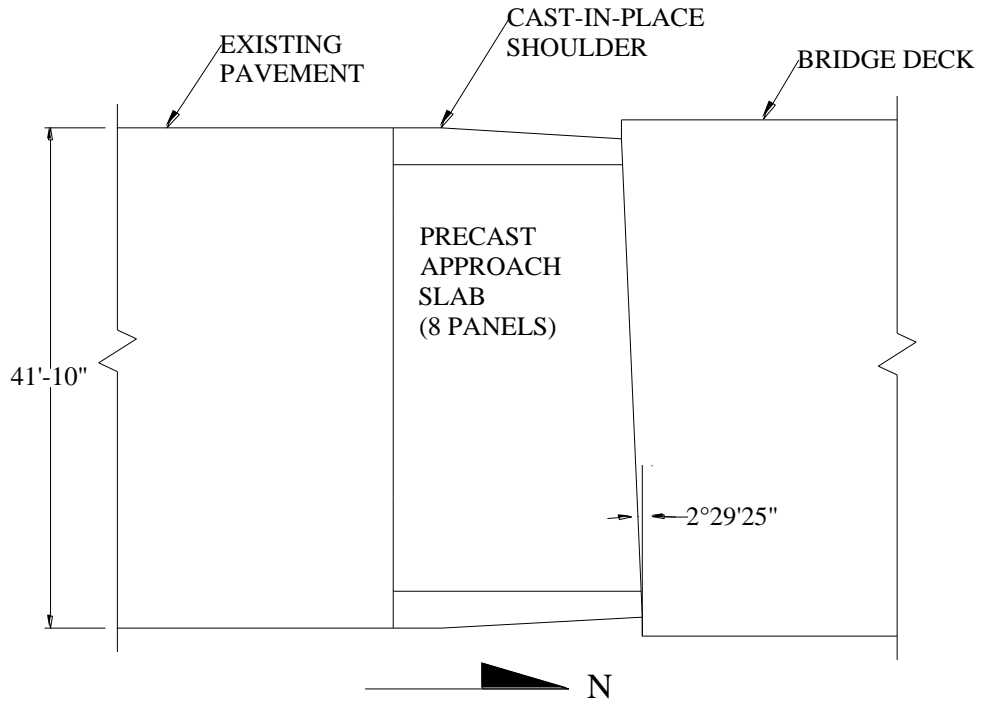
Figure 3.1. Plan view of precast approach slab with bridge and existing pavement (see Figure 3.2 for slab panel dimensions)
