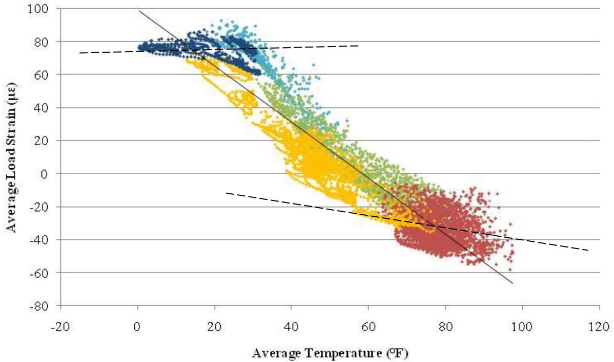
Figure 4.20. Average load strain with respect to average slab temperature
