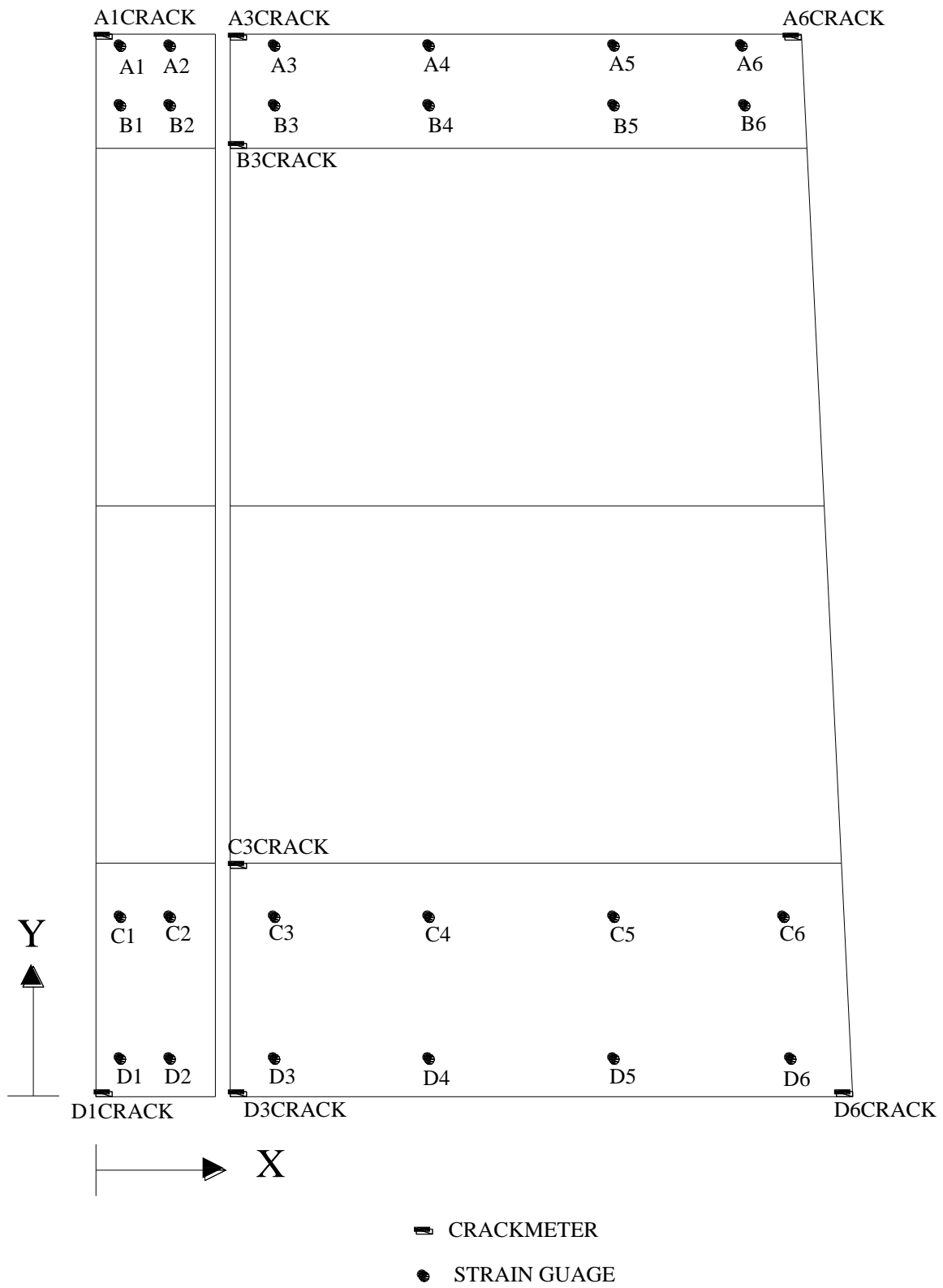
Figure 3.5. Instrumentation layout
