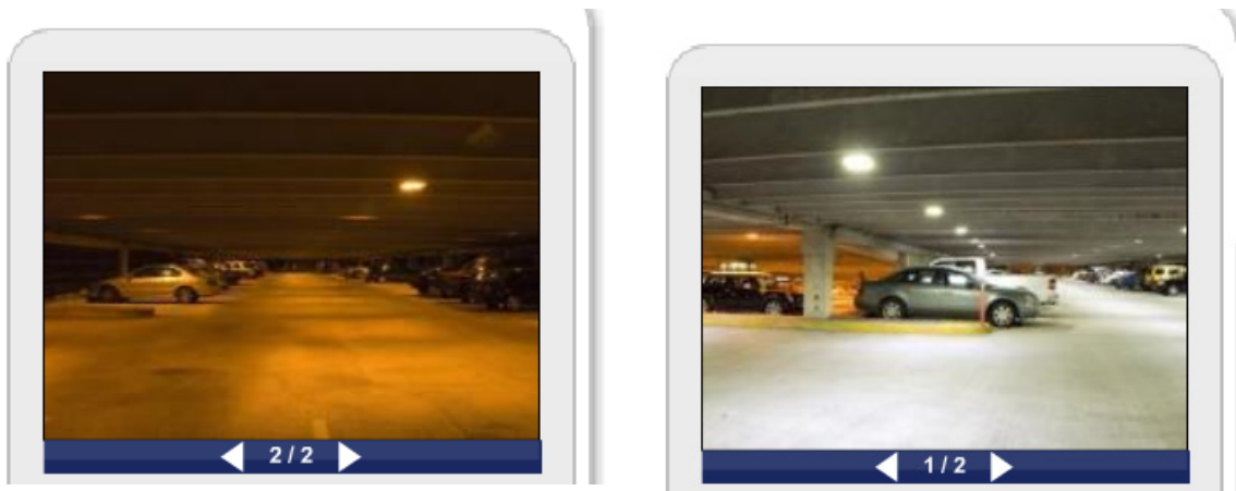
Figure 5-8: Application of LED Lighting in Parking Deck (before LED—left, After LED lighting was installed—right (Image source: WRAL, 2007)
