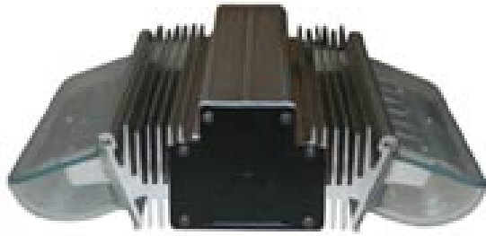
Figure 5-5: IntenCity Luminaire (image source: IntenCity, 2007)
