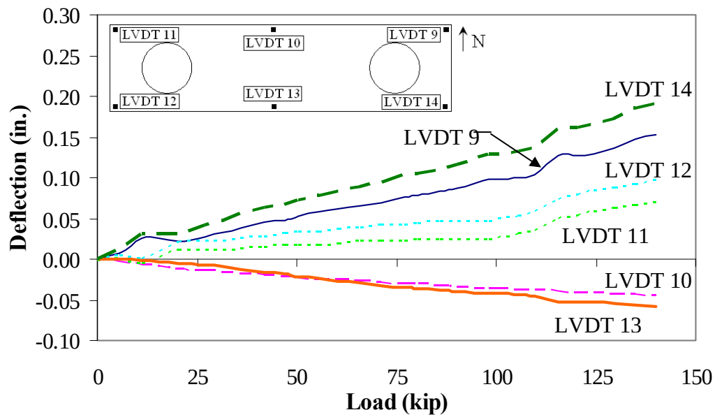
Figure 71. Total deflection of ADC1
