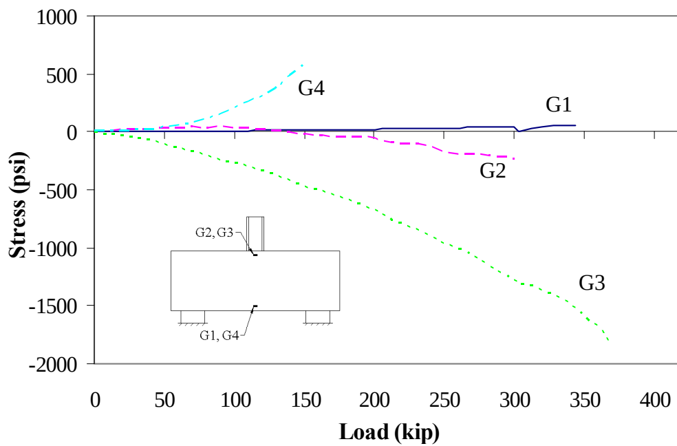
Figure 172. Concrete stress for Shear Test 4
