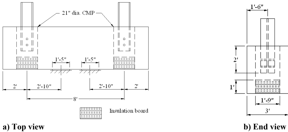
Figure 30. Double pile abutment test specimen
