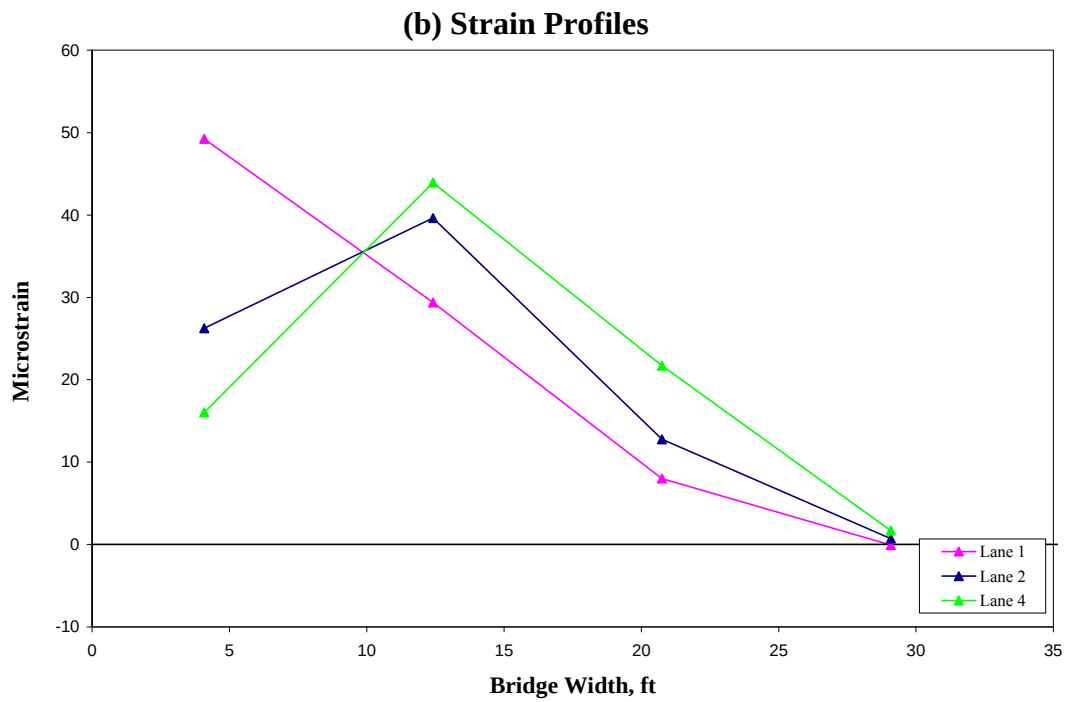
Figure 3.4 MS 2 Strain and Deflection Profiles (Load Case 3)
