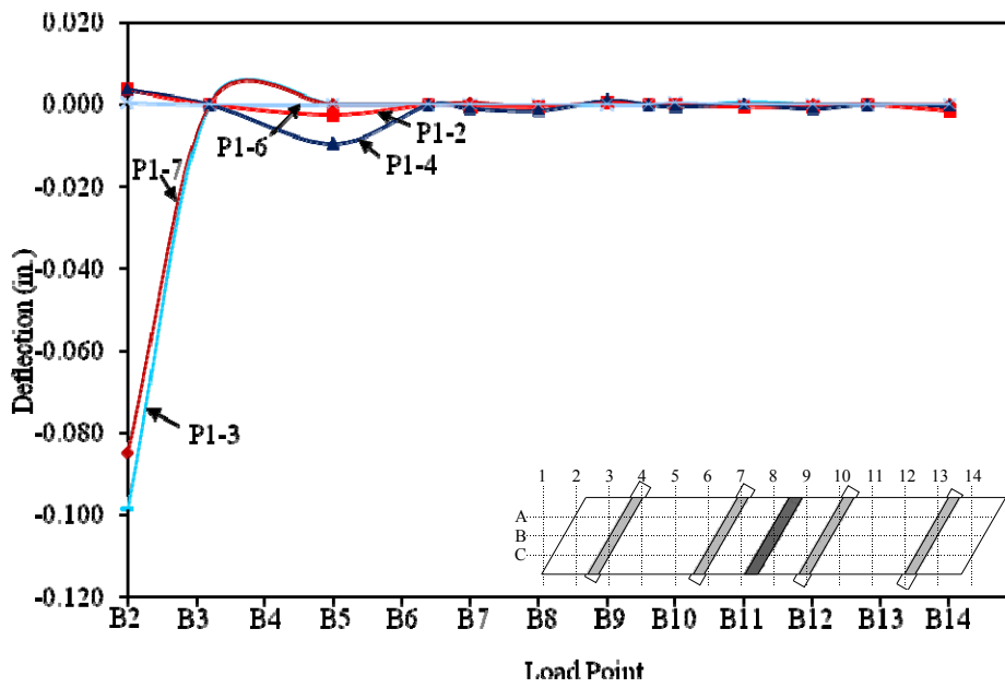
a) Panel 1 deflections
