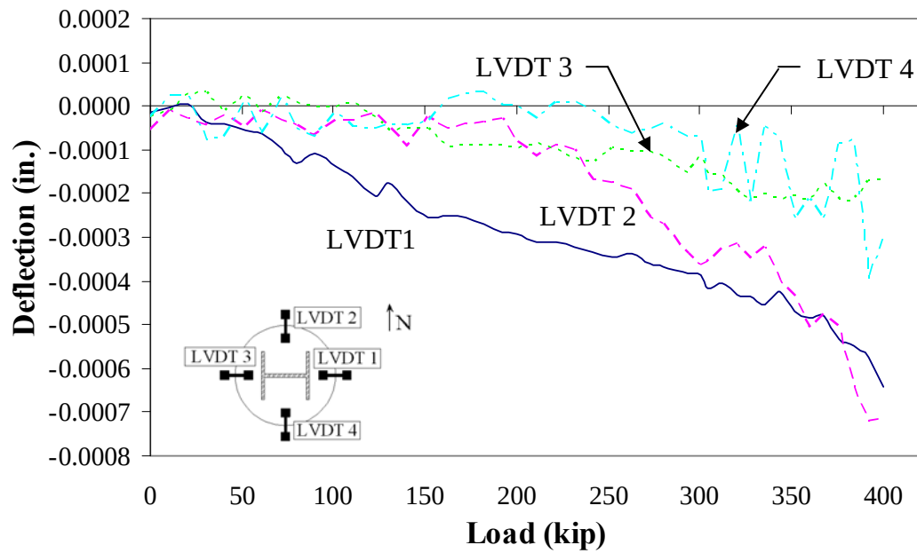
Figure 170. Top deflection for Shear Test 3
