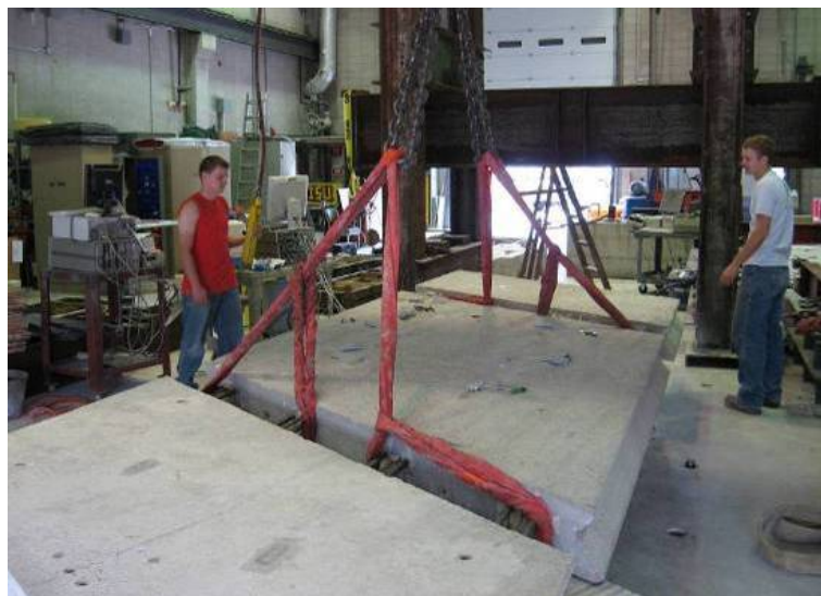
a) Photograph of lifting the deck panel with four straps
