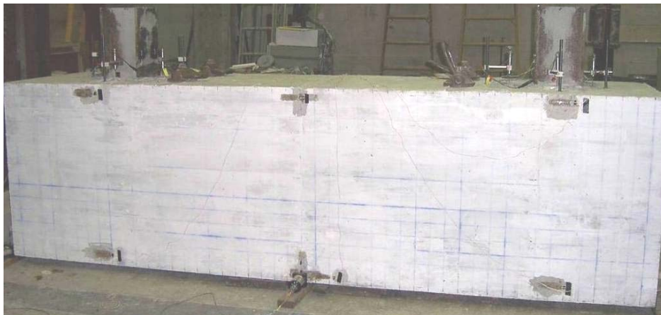
Figure 41. Instrumentation on an ADC1 prior to testing
