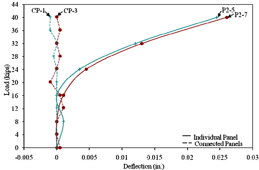
c) Deflections P2-5, P2-7, CP-1, and CP-3
