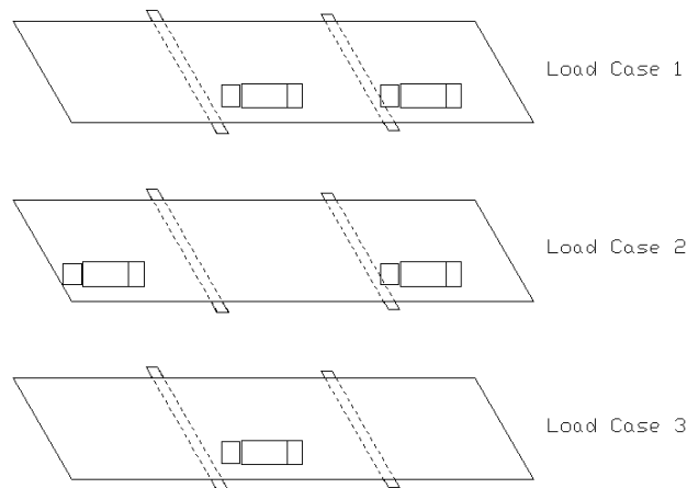
Figure 2.14 Load cases for static tests
