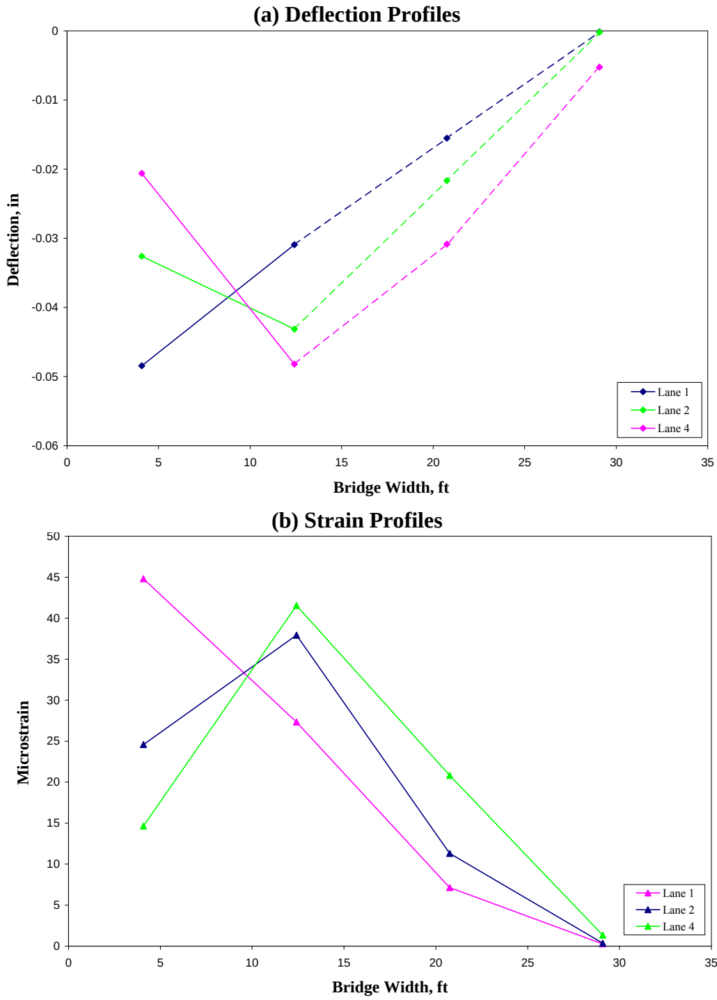
Figure 3.2 MS 2 Strain and Deflection Profiles (Load Case 1)
