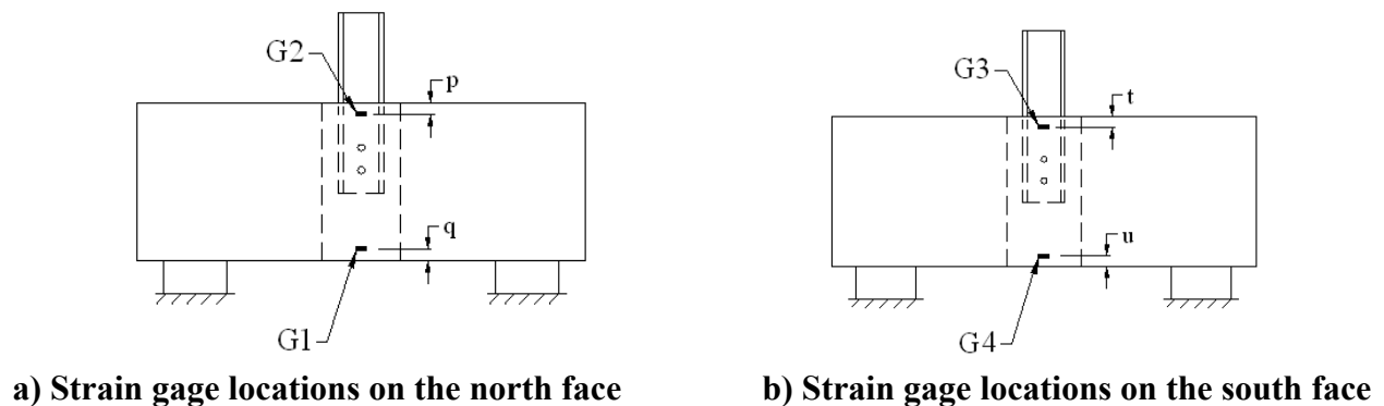
Figure 44. Single pile specimens: locations of strain gages on concrete.
