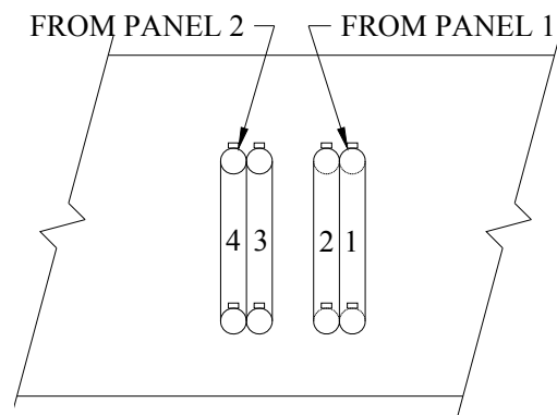
□ = STEEL STRAIN GAGE d) Section B-B
