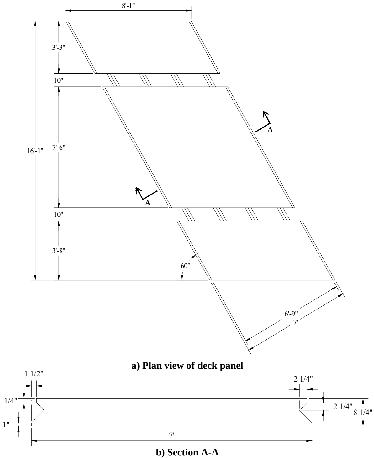
Figure 2.2. Deck panel dimensions
