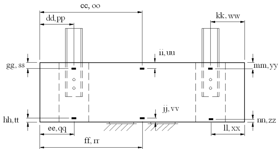
c) Locations of the strain gages (north and south face)
