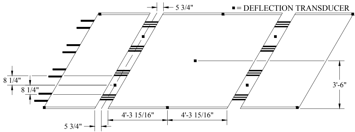
a) Location of deflection measurements
