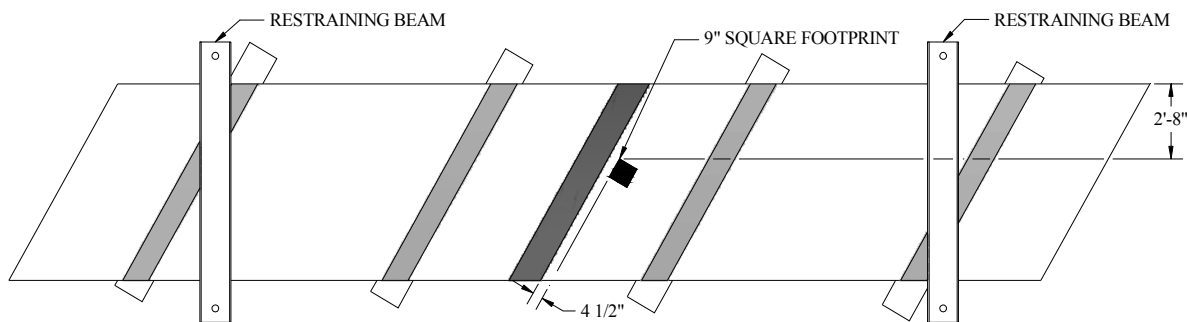
a) Location of 9 in. square footprint
