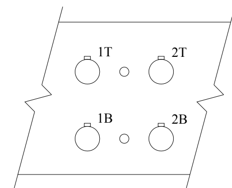
□ = STEEL STRAIN GAGE c) Section A-A
