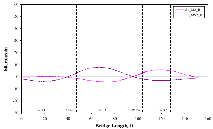
Figure 3.11 Girder 2 Strain History (Lanes 1-4)
