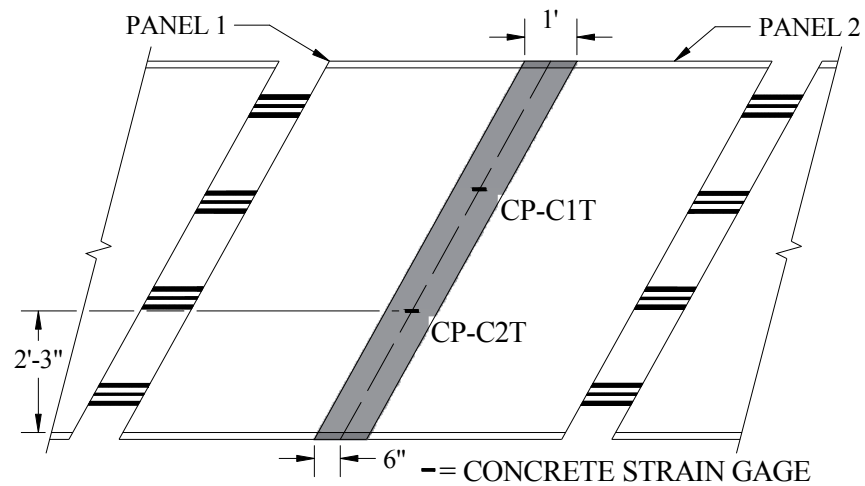
c) Closure pour concrete strain location numbering system
