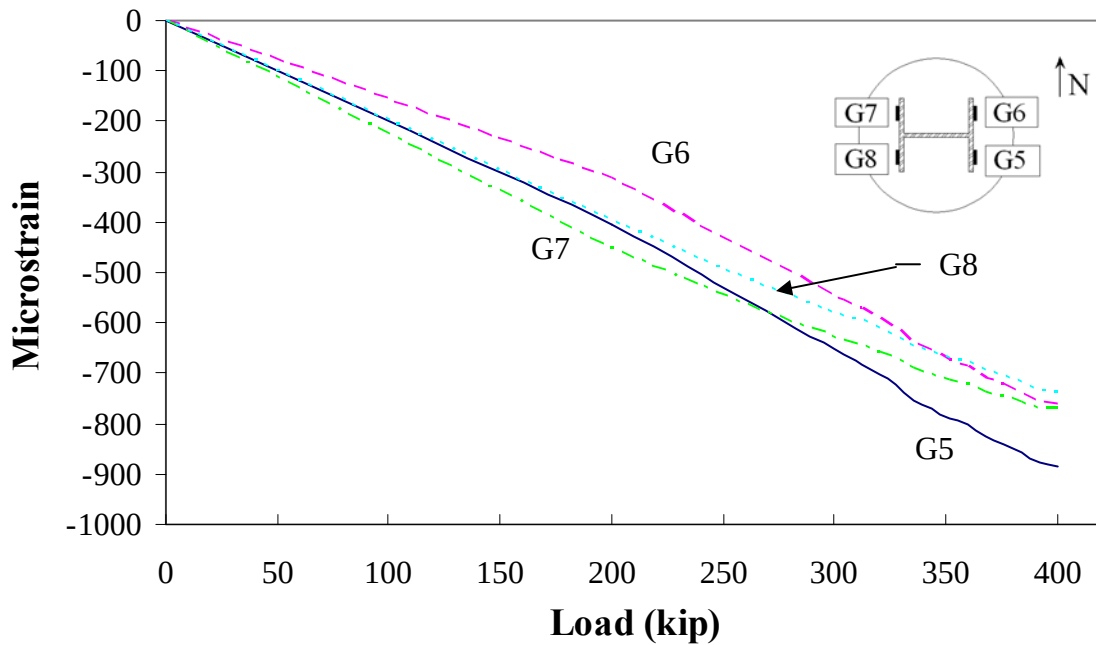
Figure 168. Steel strain for Shear Test 3
