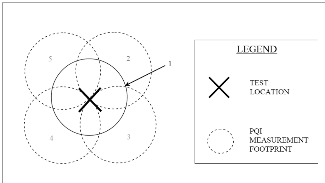
Figure 11. Schematic layout of PQI measurement sequence (New York State DOT 2003)
