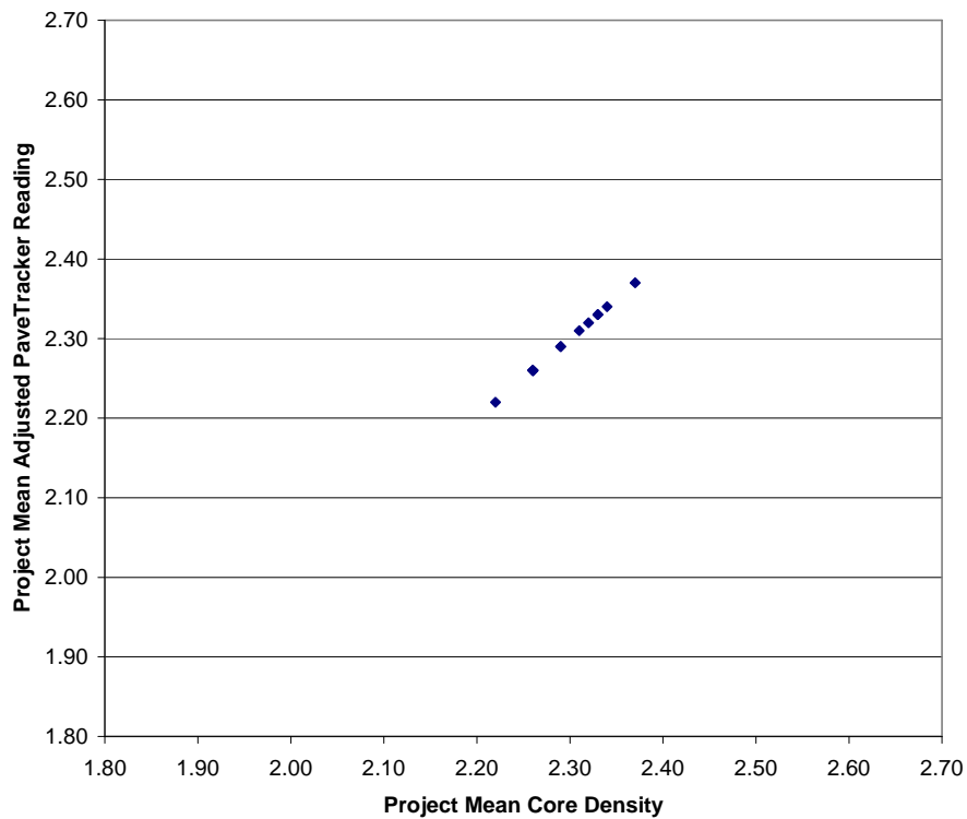
Figure A.7. Core density (g/cm 3 ) versus adjusted Pavetracker readings
