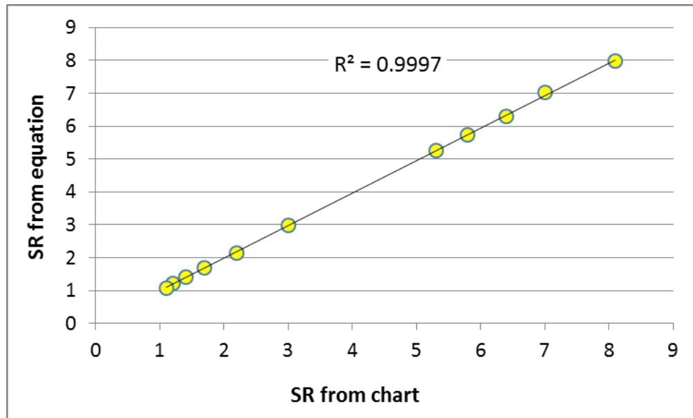
Figure 10. SR determination for rigid and composite pavements: chart versus equation
