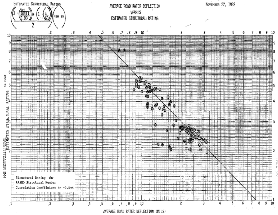
Figure 9. Rigid and composite pavement base relationship between SR and Road Rater D 0 (adapted from Potter and Dirks 1989)
