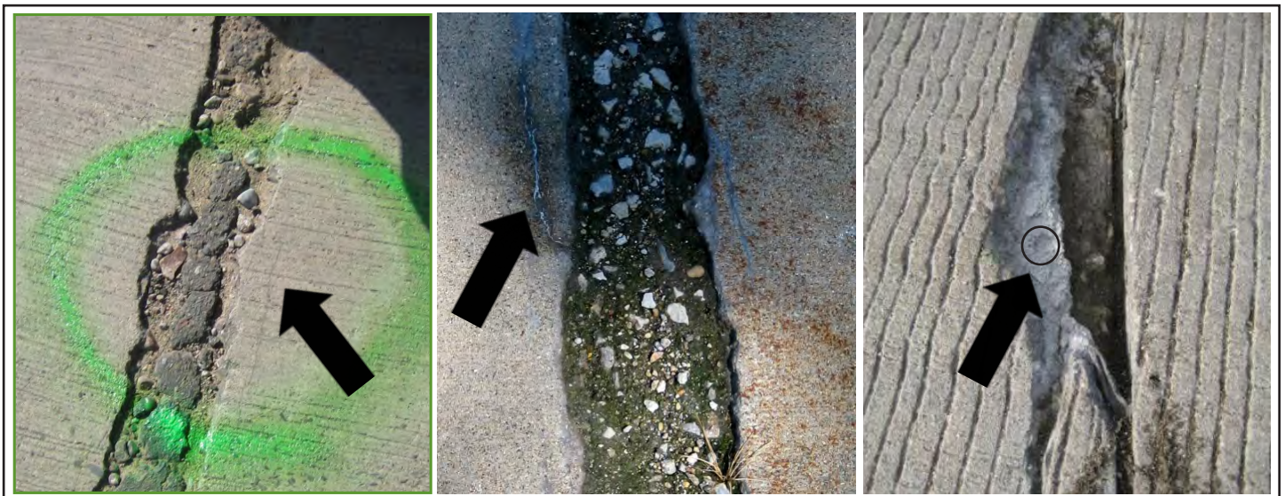
Figure 9. Typical incremental cracking: Note (left to right) the crack parallel to the ready-patched face, the signs of water passing through the crack, and the exposed aggregate remaining in the concrete
