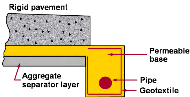
Figure 34. Typical components of an edge drain system (Source: NHI 131008) (16)
