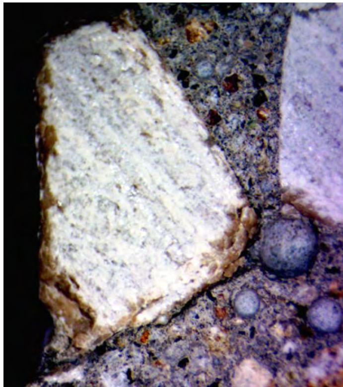
Figure 15. Photograph of an aggregate particle dislodged by inappropriate sawing (Field of view 5mm)
