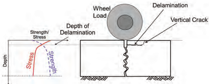
Figure 17. Early-aged drying stresses (left) and resulting horizontal cracking and delamination spalling (right) due to high moisture loss during placement (2)
