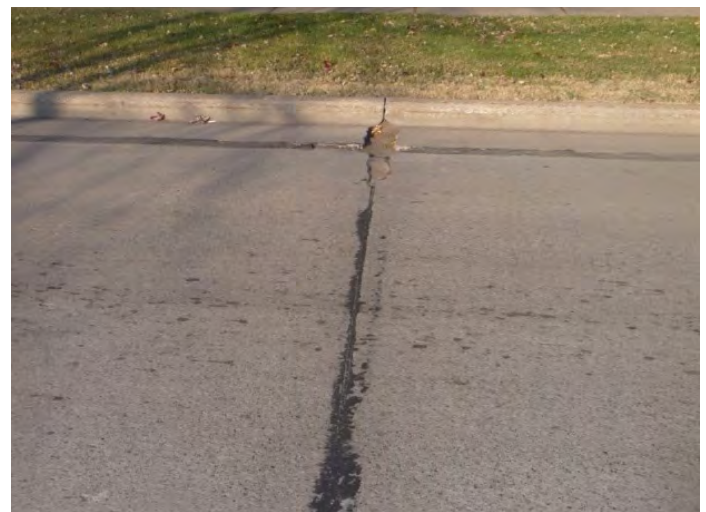
Figure 33. Failing transverse joint associated with poor drainage at gutter
