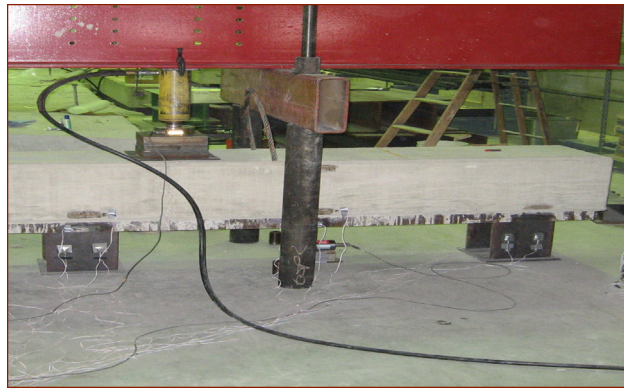
Laboratory testing on a precast abutment cap
