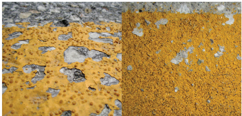
Sample material loss (loss of presence) on waterborne paint products after two winters
