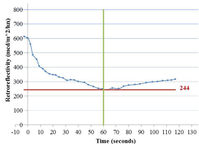
Sample wet retroreflectivity measurements (shown in blue), indicating the amount of loss that the driver sees, with the initial dry readings (two) at above 600 mcd/m 2 /lux and the wet readings down to less than half of that, at 244 (red line), after one minute of wetting (green line)
