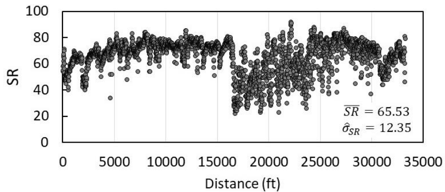
Figure 41. SCRIM readings acquired at prevailing traffic speed from curves Mis1 through Mis4
