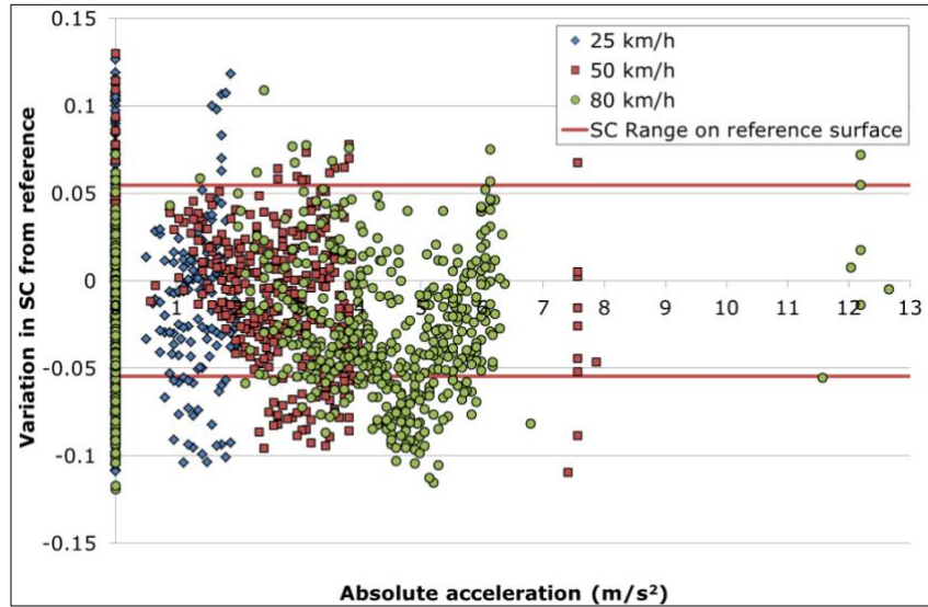
Figure 10. SCRIM variation from reference
