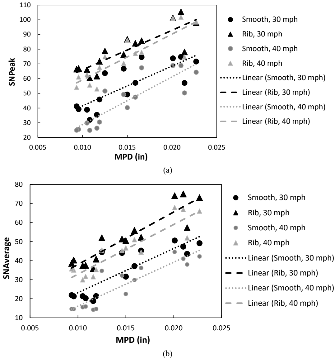
Figure 31. Scatter plots with fitted linear regression models of (a) peak and (b) average SNs versus the MPD values acquired using stationary LTS
