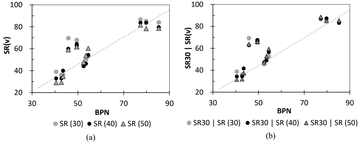
Figure 36. SCRIM measurements acquired at the three nominal speeds plotted against the BPN: (a) uncorrected SCRIM readings and (b) SCRIM readings corrected to 30 mph
