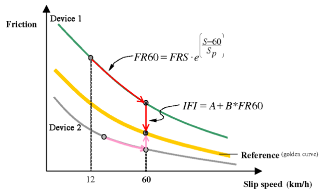
Figure 21. Demonstration of the IFI
