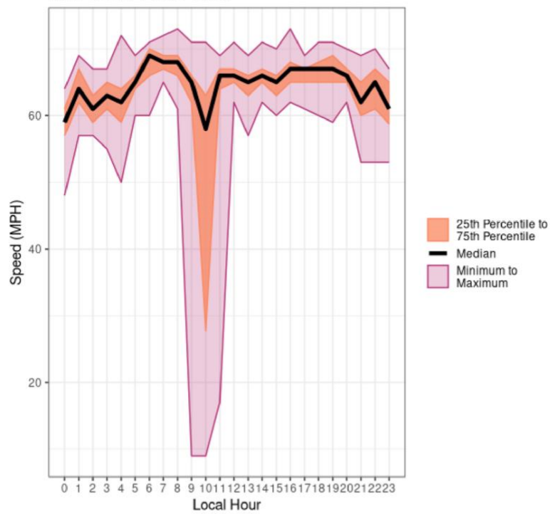
Summaries of Work Zone Speeds (MPH) during Peak Periods from INRIX Probe Data
